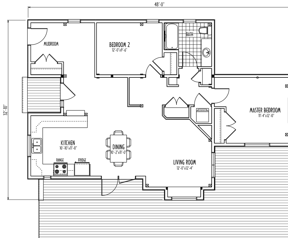
MAIN FLOOR PLAN AREA 1168 SQ.FT.
